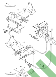
ETB-007846, Sterowanie +/- ZA-M Special (2/2)
