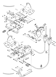
ETB-007845, Sterowanie +/- ZA-M Special (1/2)
